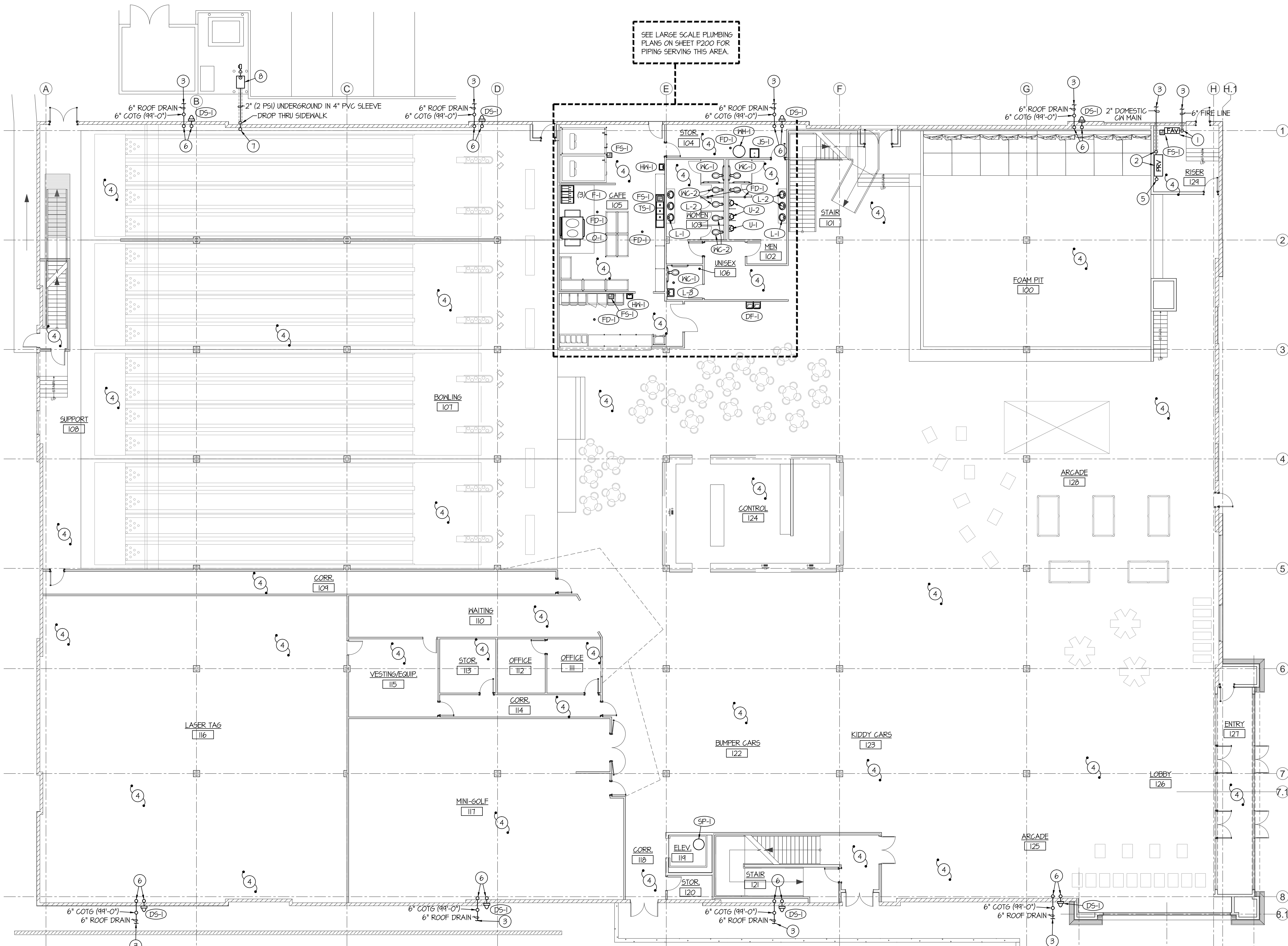
PLUMBING FLOOR PLAN SCALE: 3/32" = 1'-0"
